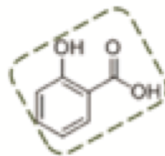
Salicylic acid
