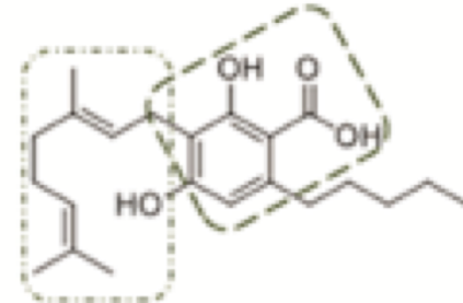
CBGA
