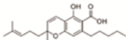
CBCA
